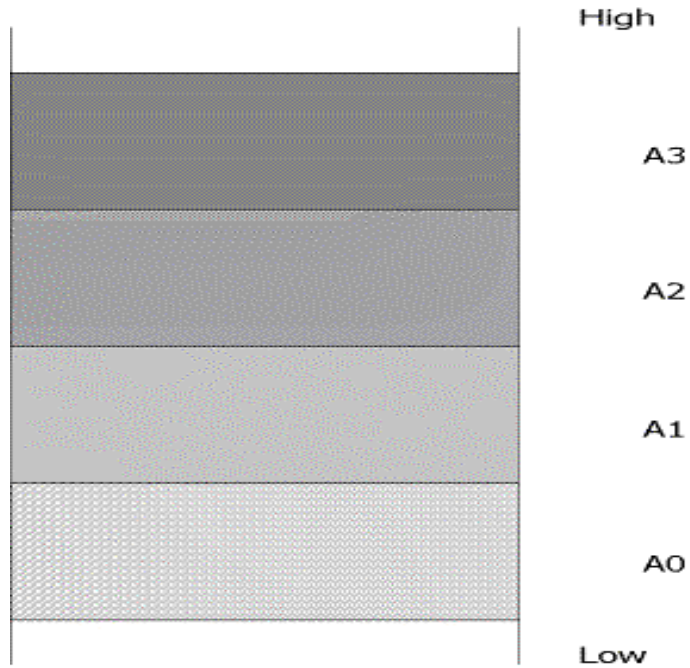
Figure 5: Block buffers
