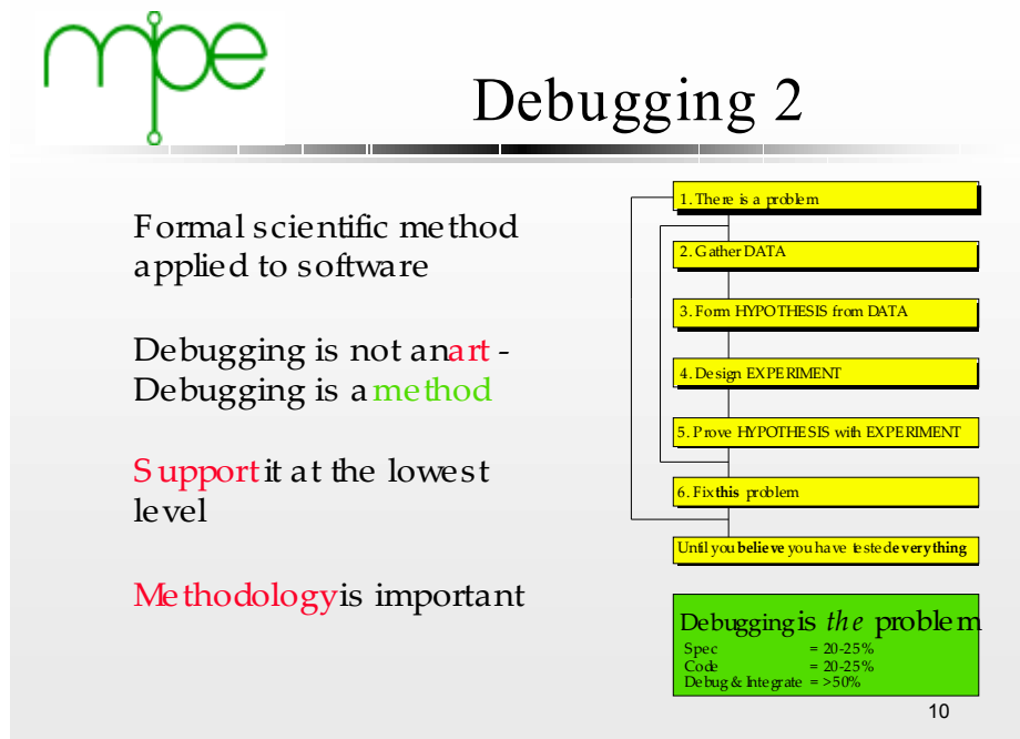
Figure 1: Debugging
